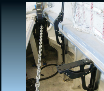
95° opening anchor locker hinge
