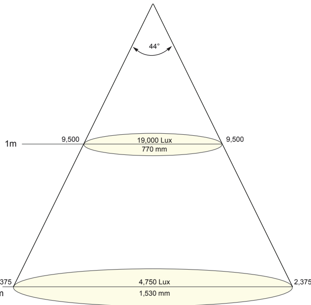
Luminous Intensity - Distance / Lux
