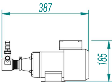
BOOSTER PUMP
